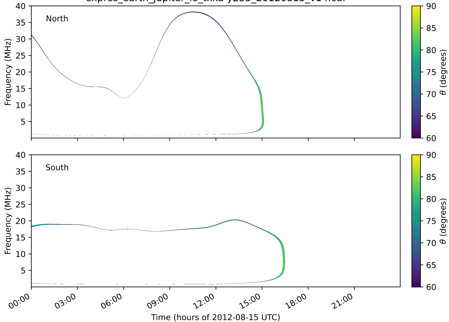
expres_earth_jupiter_io_txka-y235_20120815_v14.cdf
