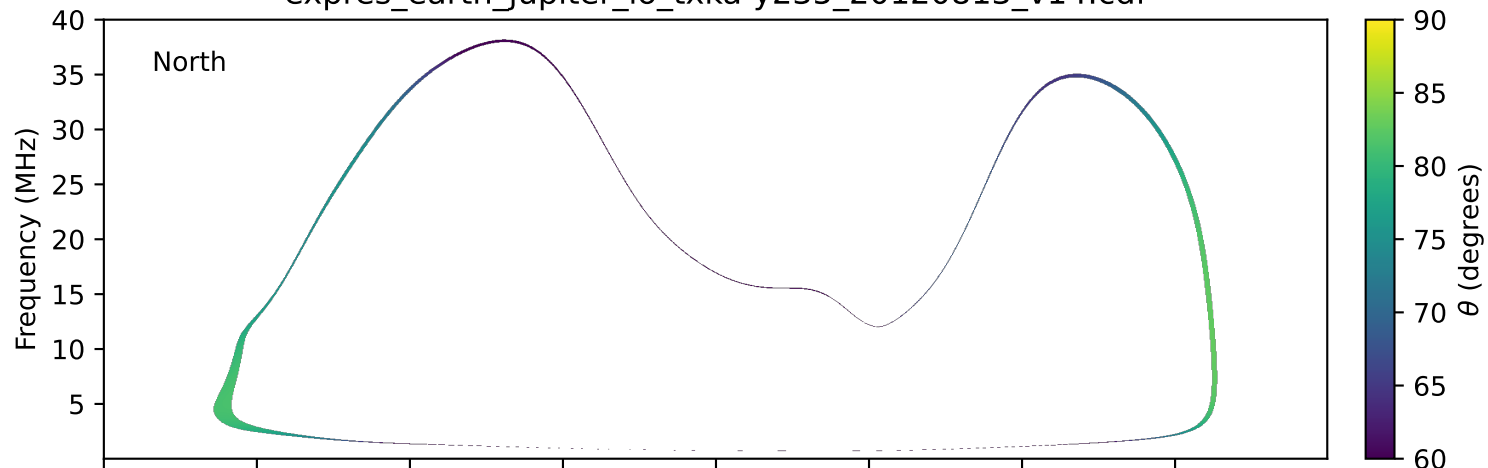
expres_earth_jupiter_io_txka-y235_20120813_v14.cdf
