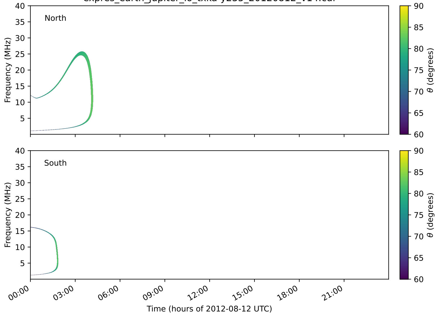
expres_earth_jupiter_io_txka-y235_20120812_v14.cdf
