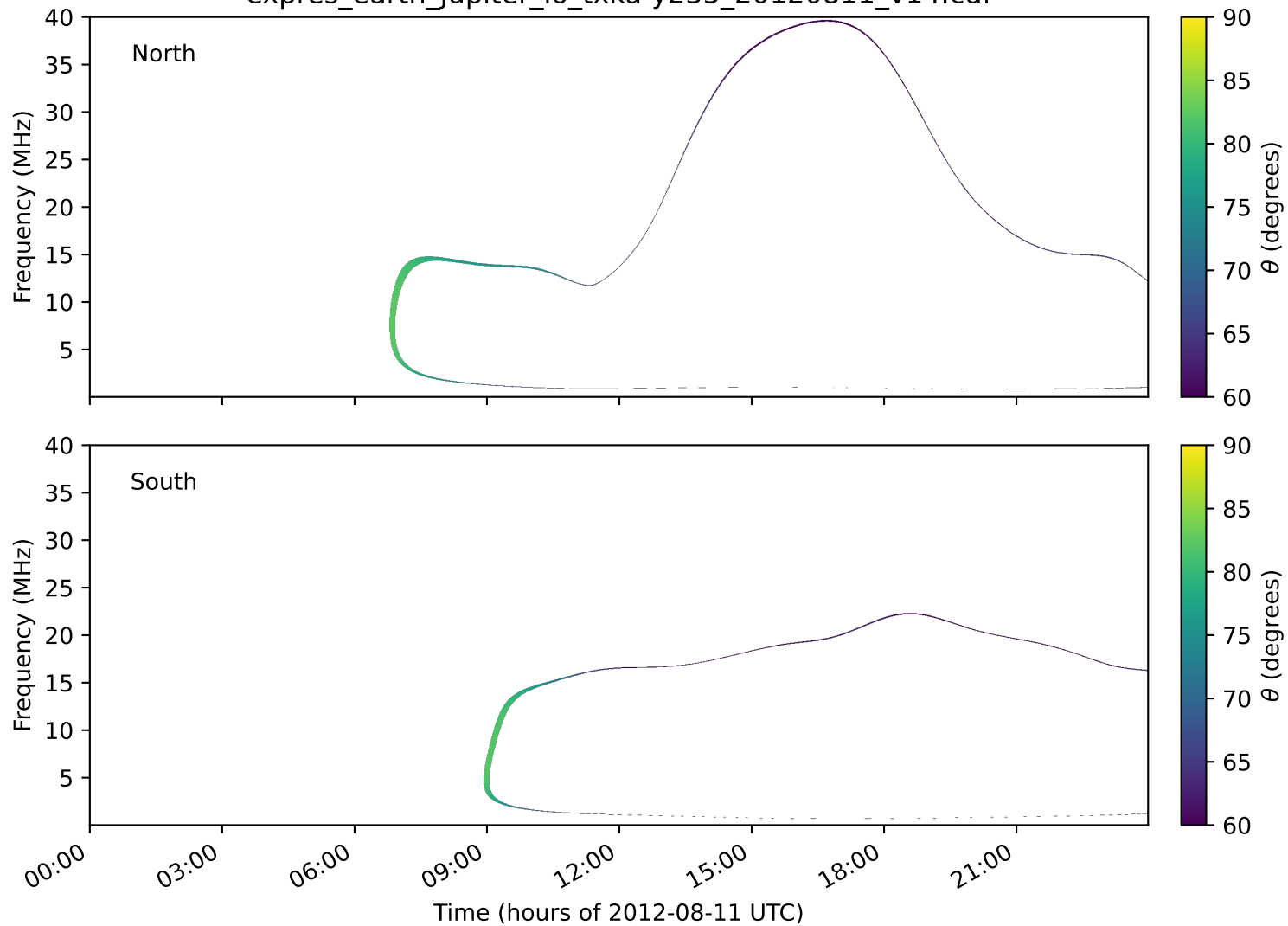
expres_earth_jupiter_io_txka-y235_20120811_v14.cdf
