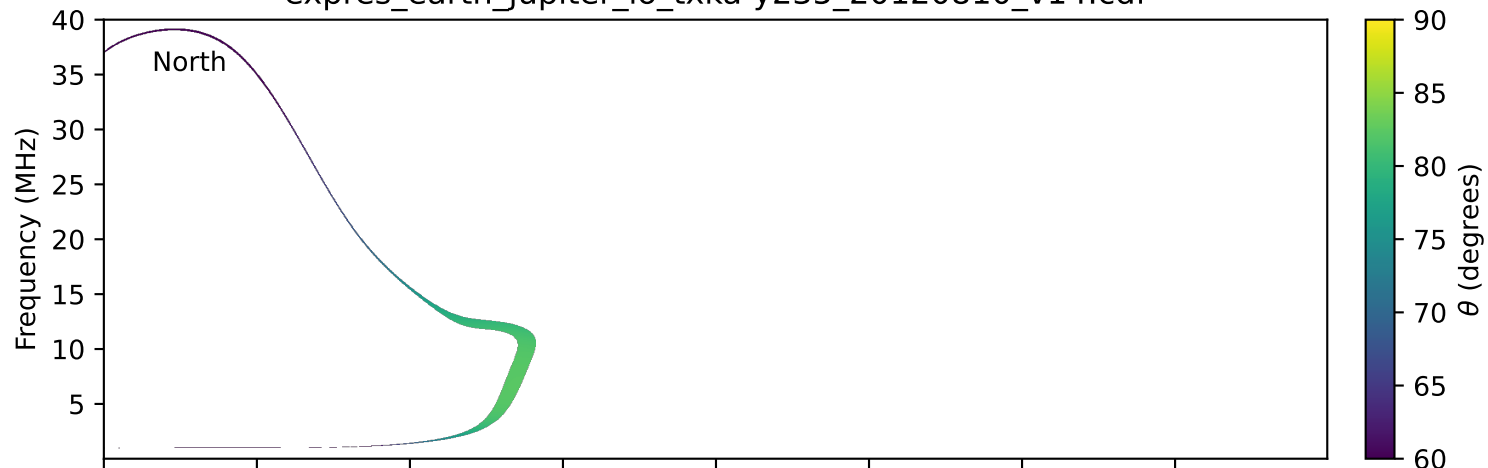
expres_earth_jupiter_io_txka-y235_20120810_v14.cdf
