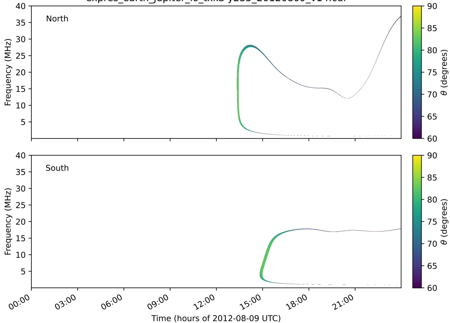
expres_earth_jupiter_io_txka-y235_20120809_v14.cdf
