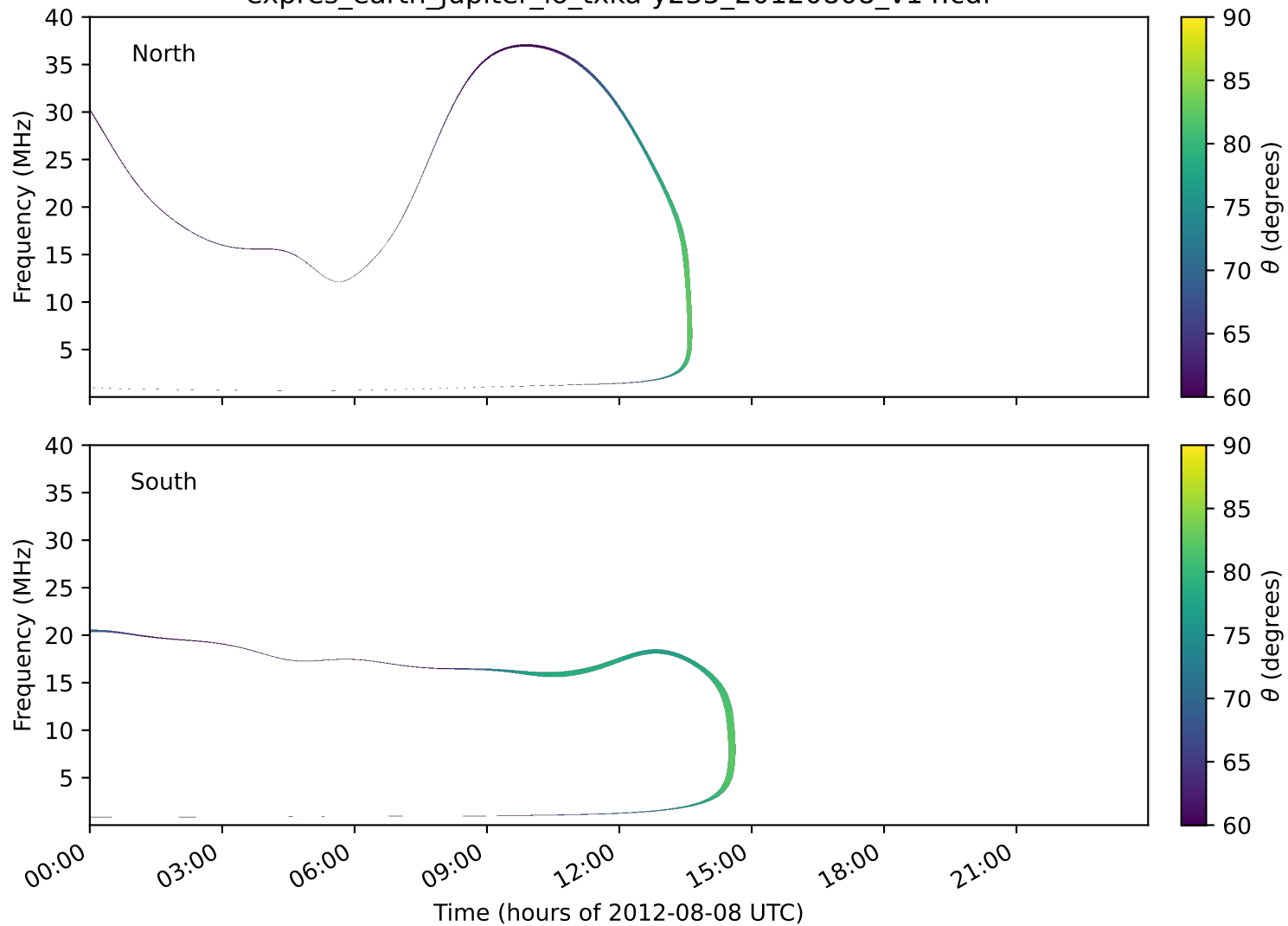
expres_earth_jupiter_io_txka-y235_20120808_v14.cdf
