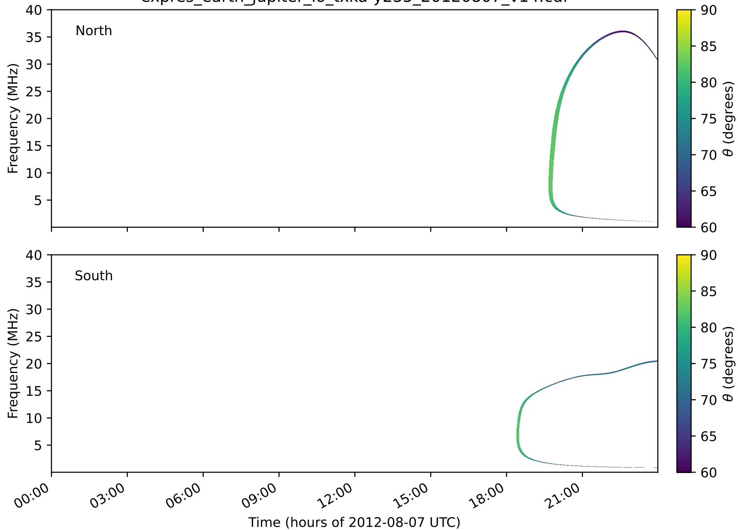
expres_earth_jupiter_io_txka-y235_20120807_v14.cdf
