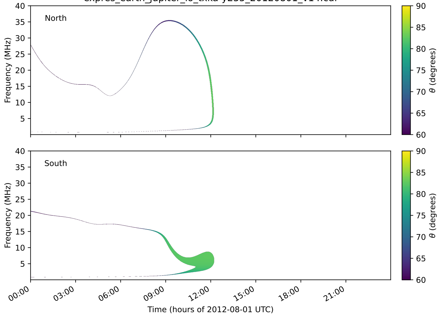
expres_earth_jupiter_io_txka-y235_20120801_v14.cdf
