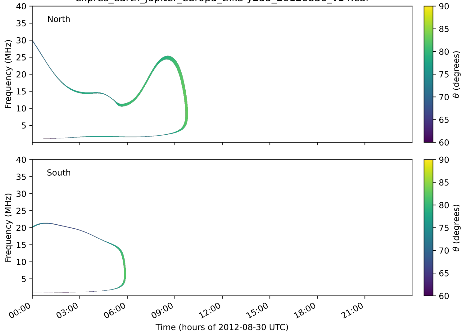
expres_earth_jupiter_europa_txka-y235_20120830_v14.cdf
