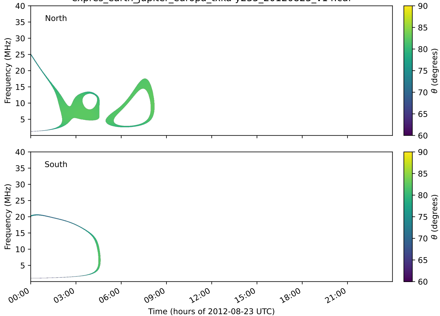
expres_earth_jupiter_europa_txka-y235_20120823_v14.cdf
