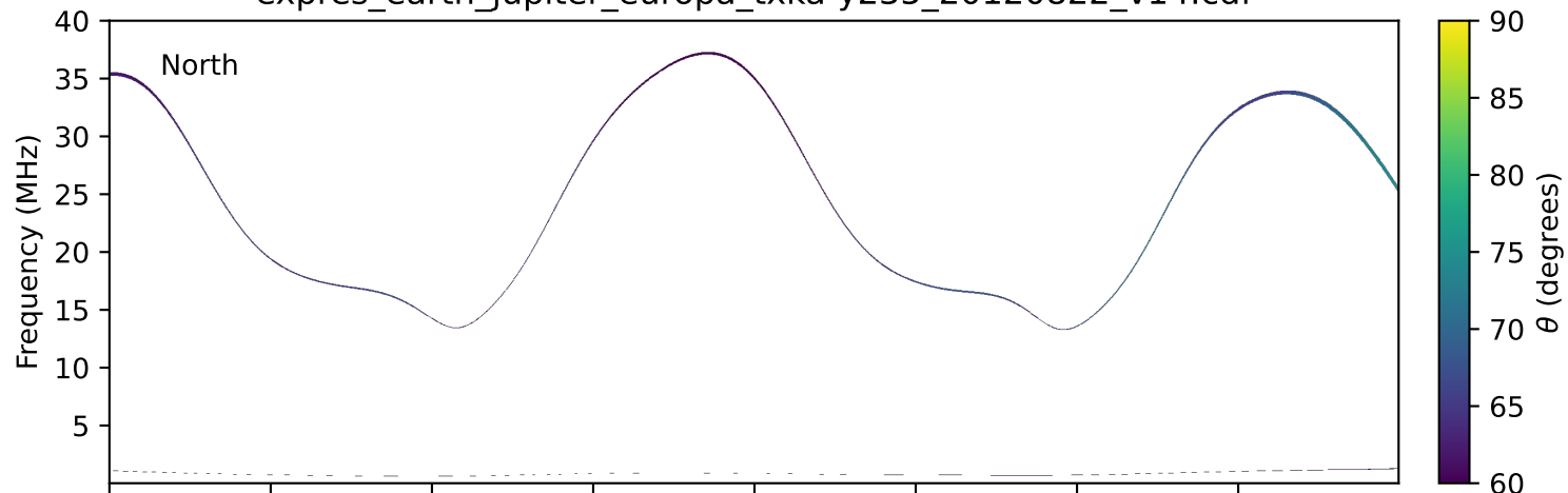
expres_earth_jupiter_europa_txka-y235_20120822_v14.cdf
