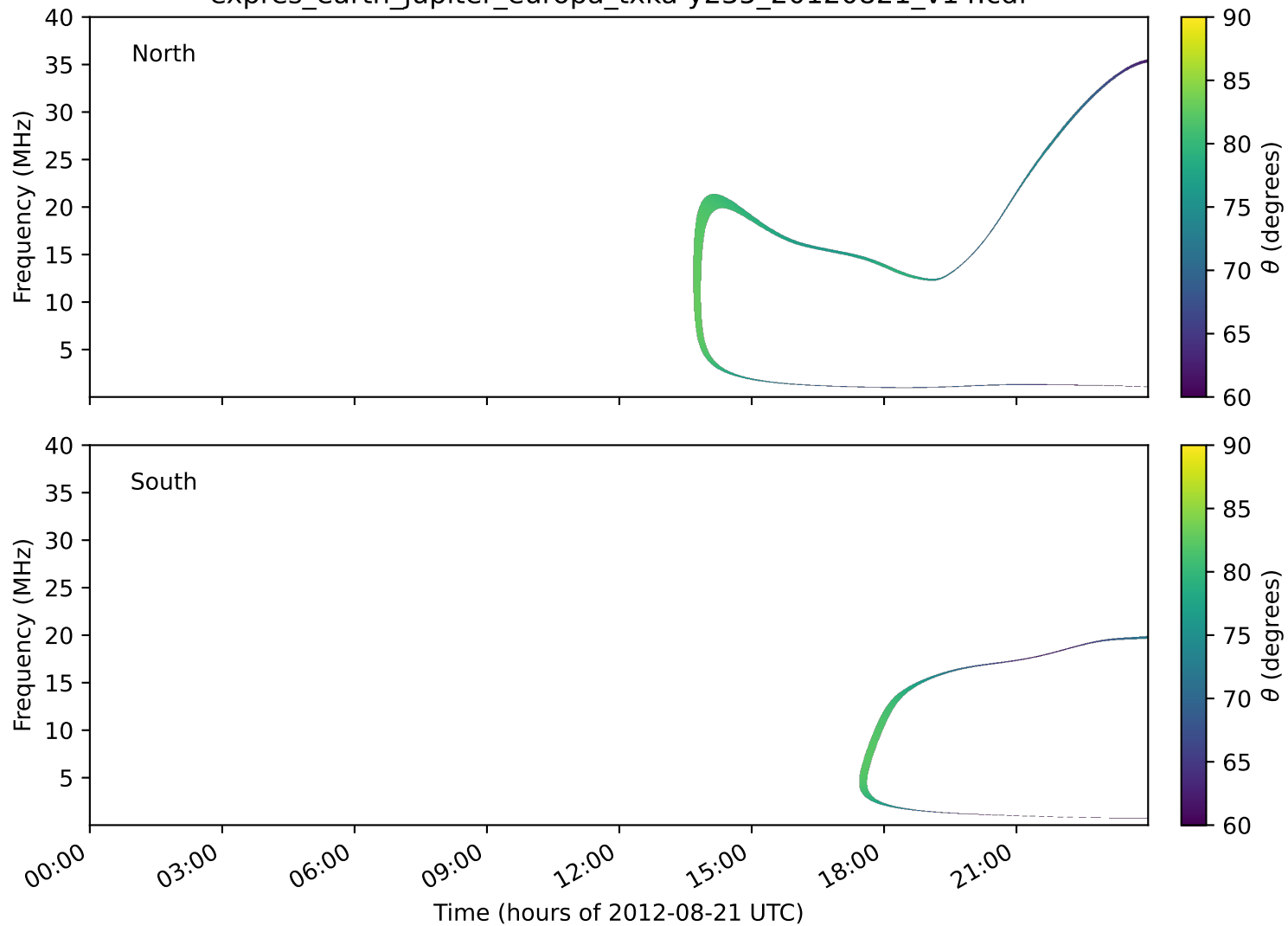
expres_earth_jupiter_europa_txka-y235_20120821_v14.cdf
