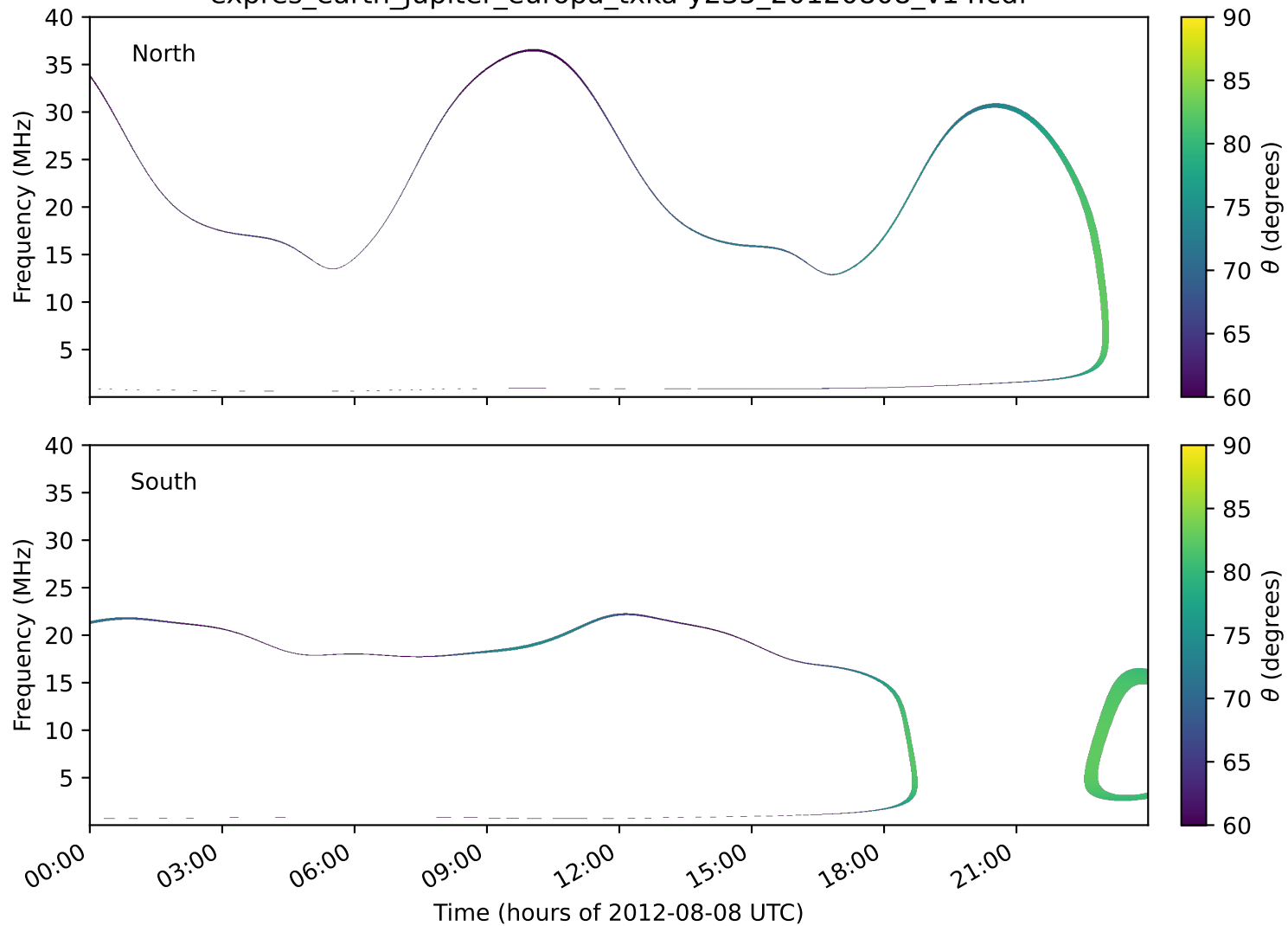
expres_earth_jupiter_europa_txka-y235_20120808_v14.cdf
