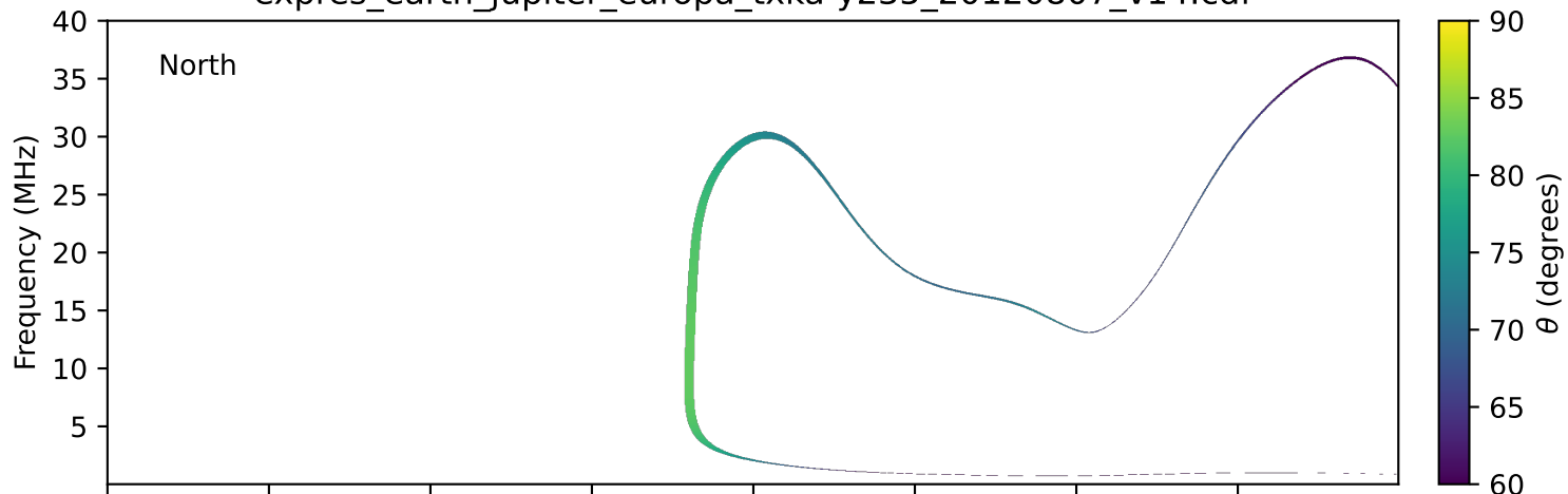
expres_earth_jupiter_europa_txka-y235_20120807_v14.cdf
