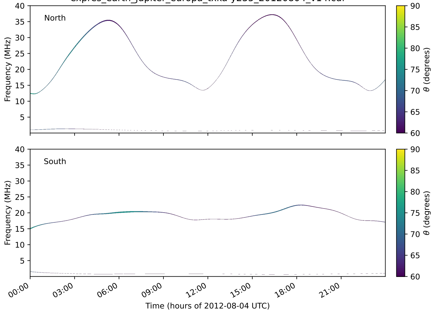
expres_earth_jupiter_europa_txka-y235_20120804_v14.cdf
