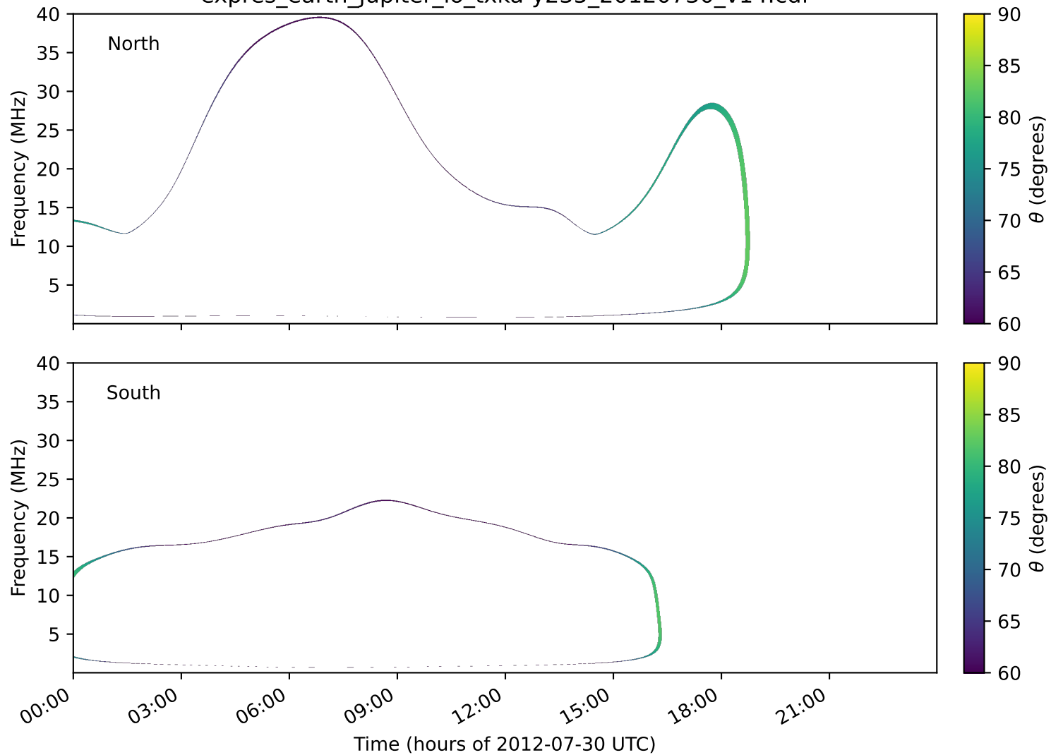
expres_earth_jupiter_io_txka-y235_20120730_v14.cdf
