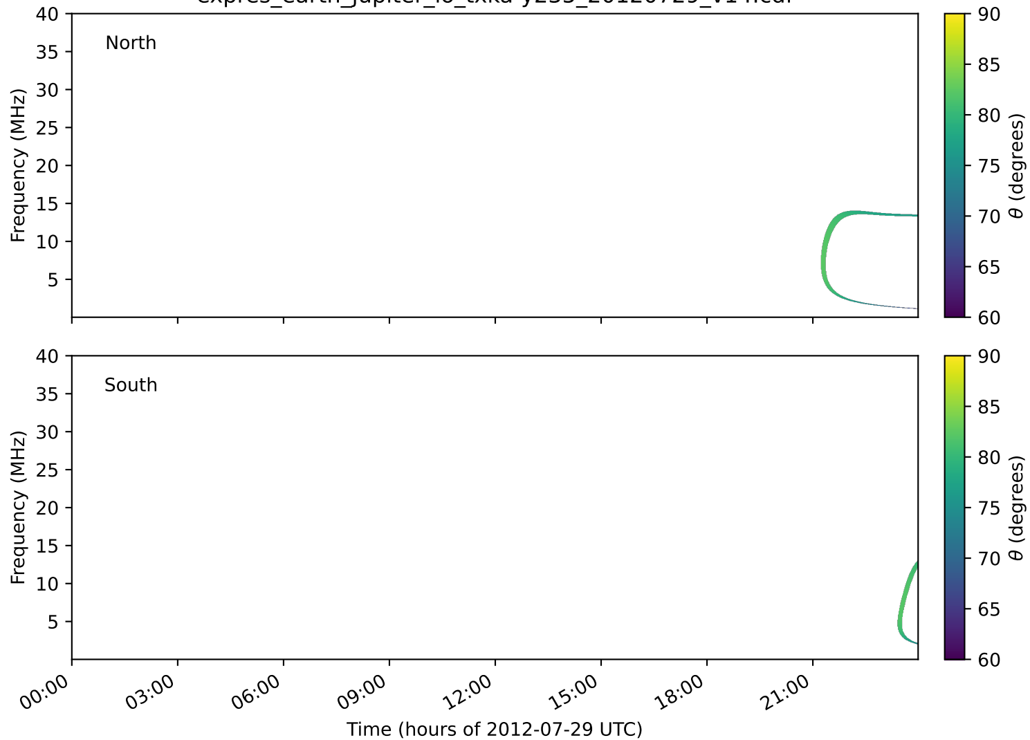
expres_earth_jupiter_io_txka-y235_20120729_v14.cdf
