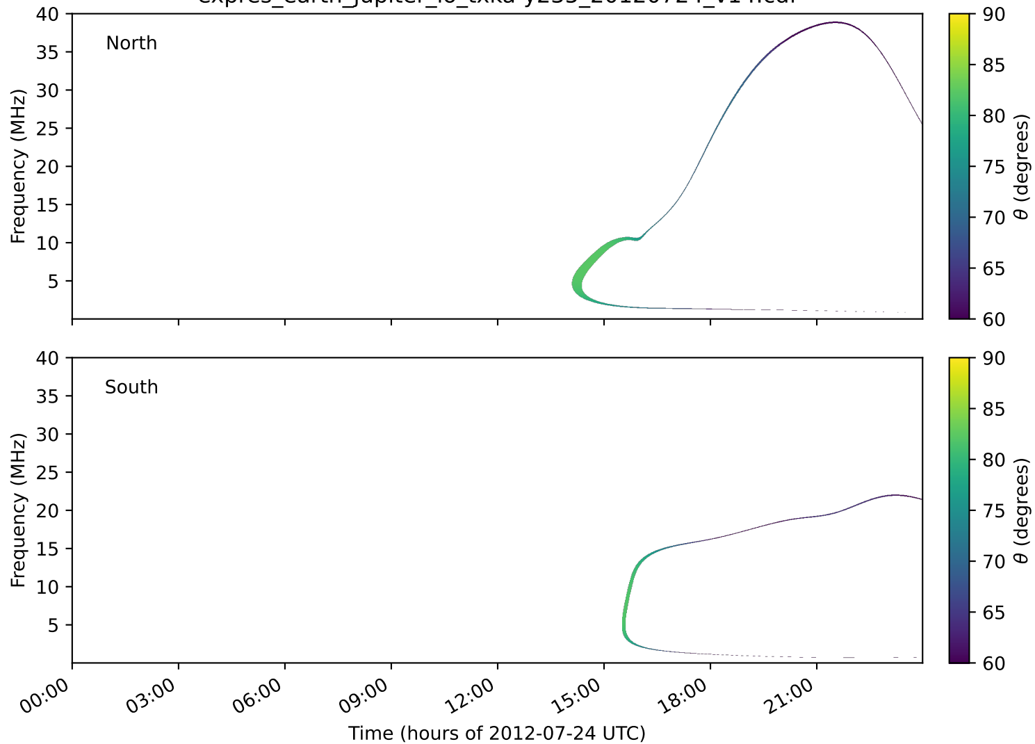
expres_earth_jupiter_io_txka-y235_20120724_v14.cdf
