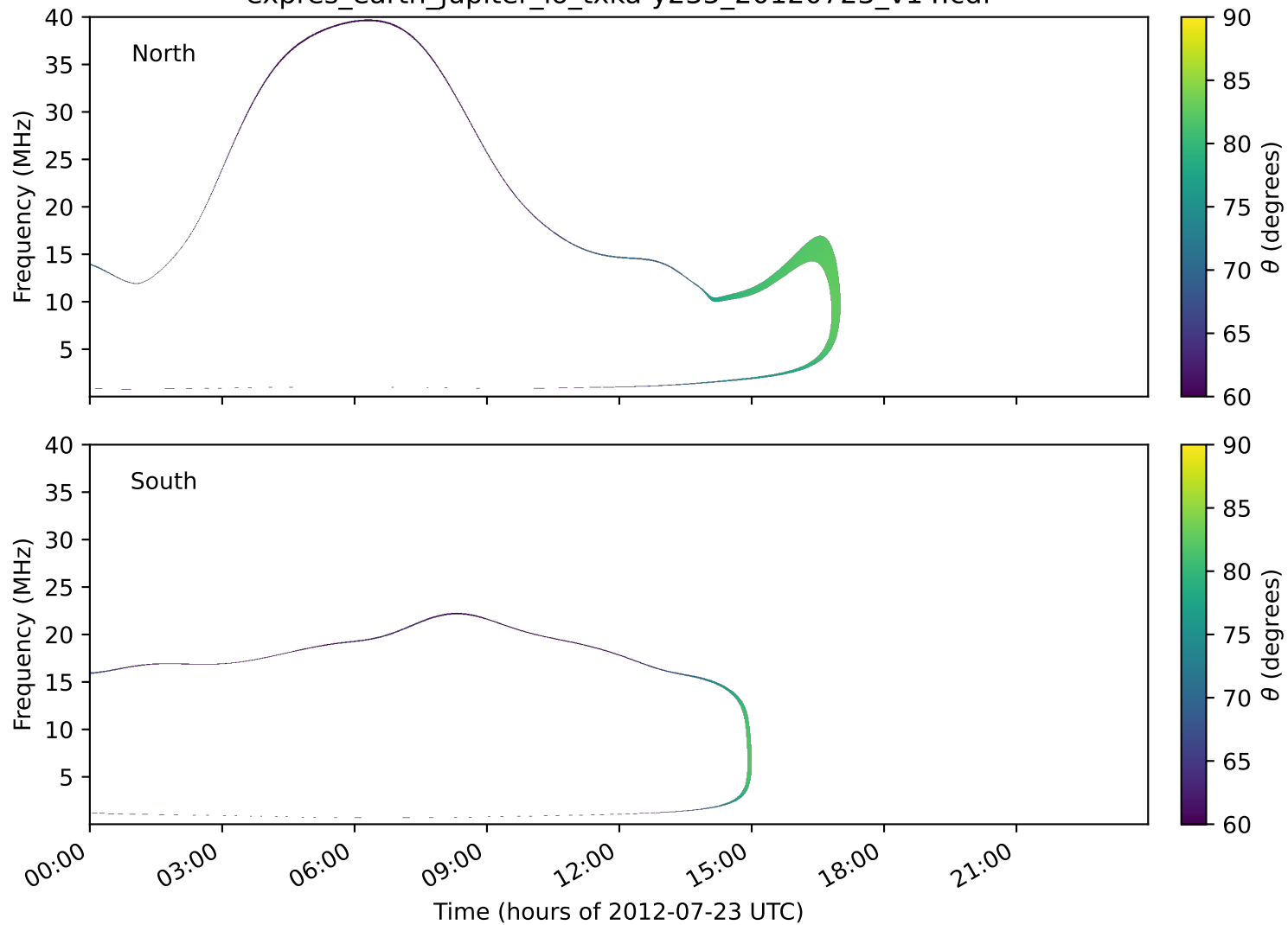
expres_earth_jupiter_io_txka-y235_20120723_v14.cdf
