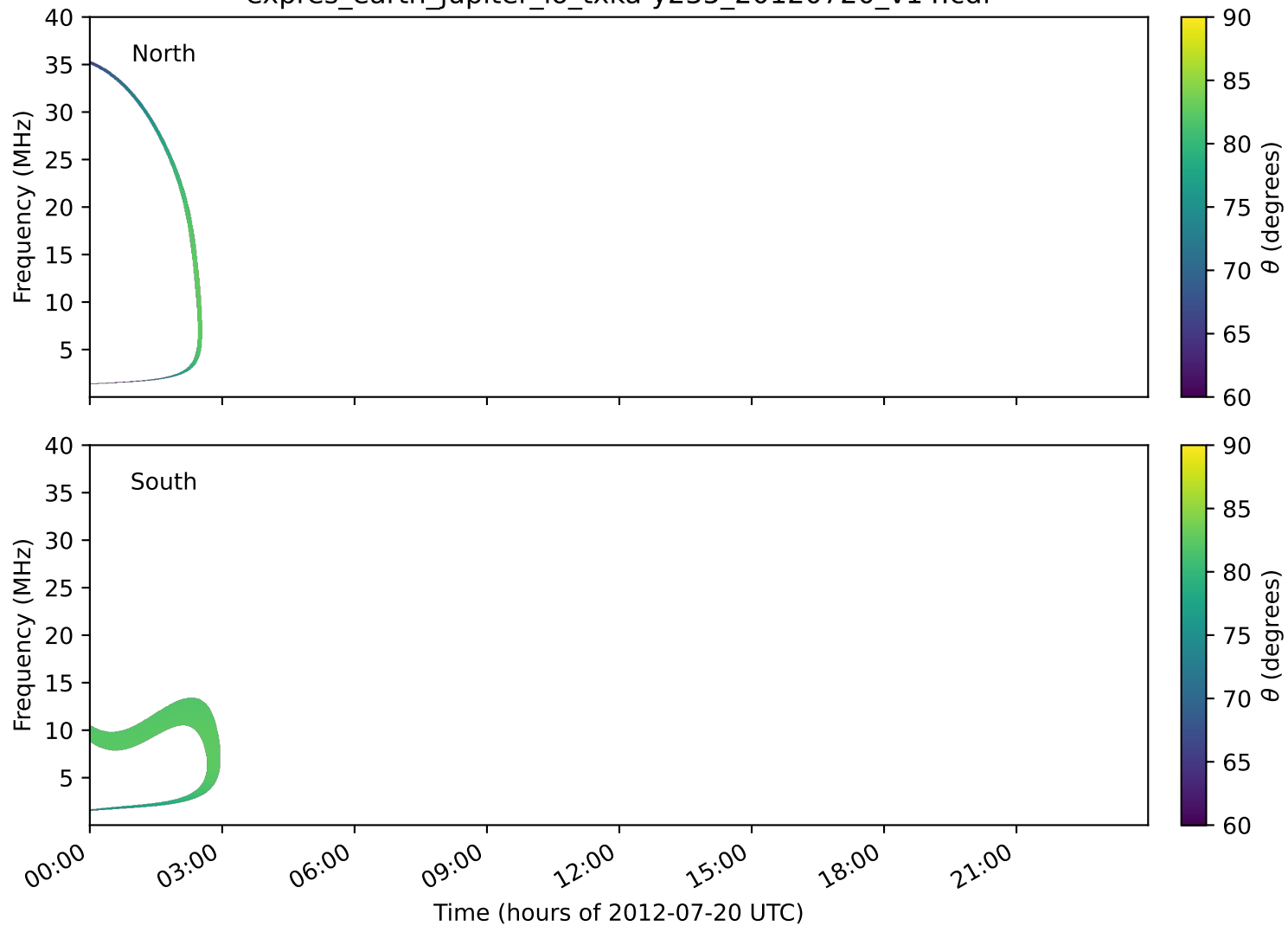
expres_earth_jupiter_io_txka-y235_20120720_v14.cdf
