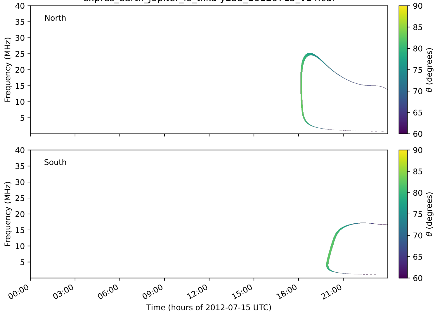
expres_earth_jupiter_io_txka-y235_20120715_v14.cdf
