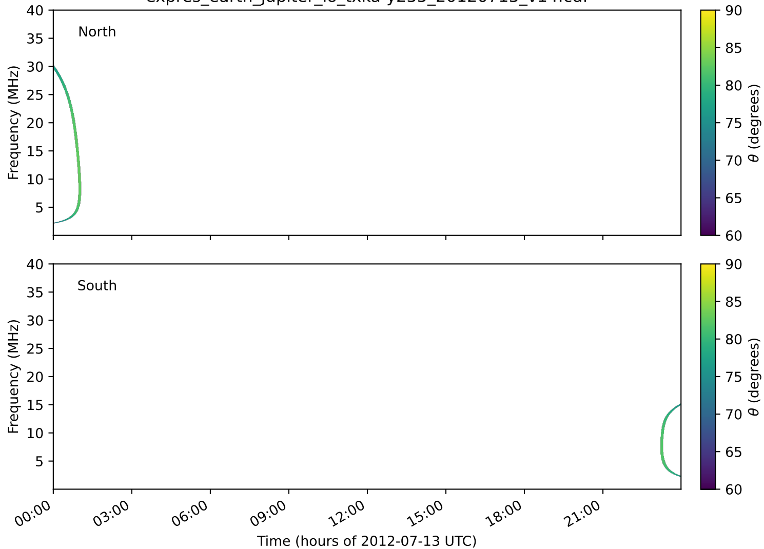
expres_earth_jupiter_io_txka-y235_20120713_v14.cdf
