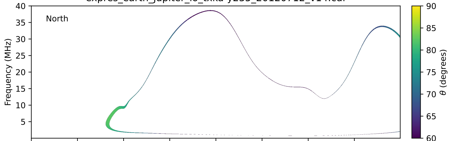
expres_earth_jupiter_io_txka-y235_20120712_v14.cdf
