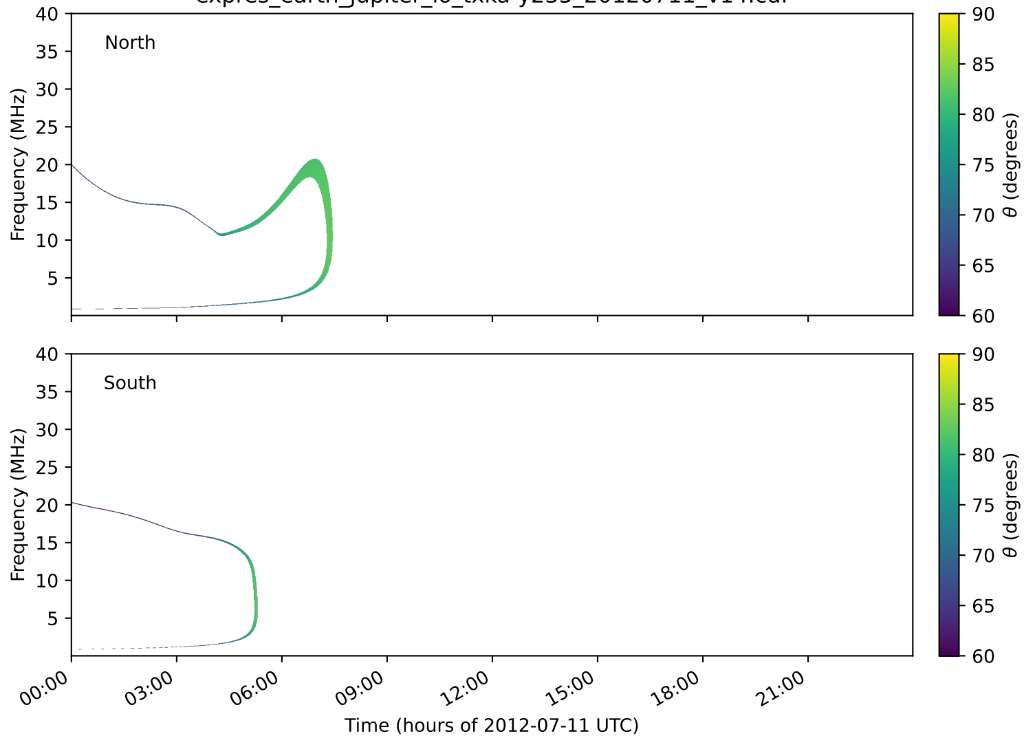
expres_earth_jupiter_io_txka-y235_20120711_v14.cdf
