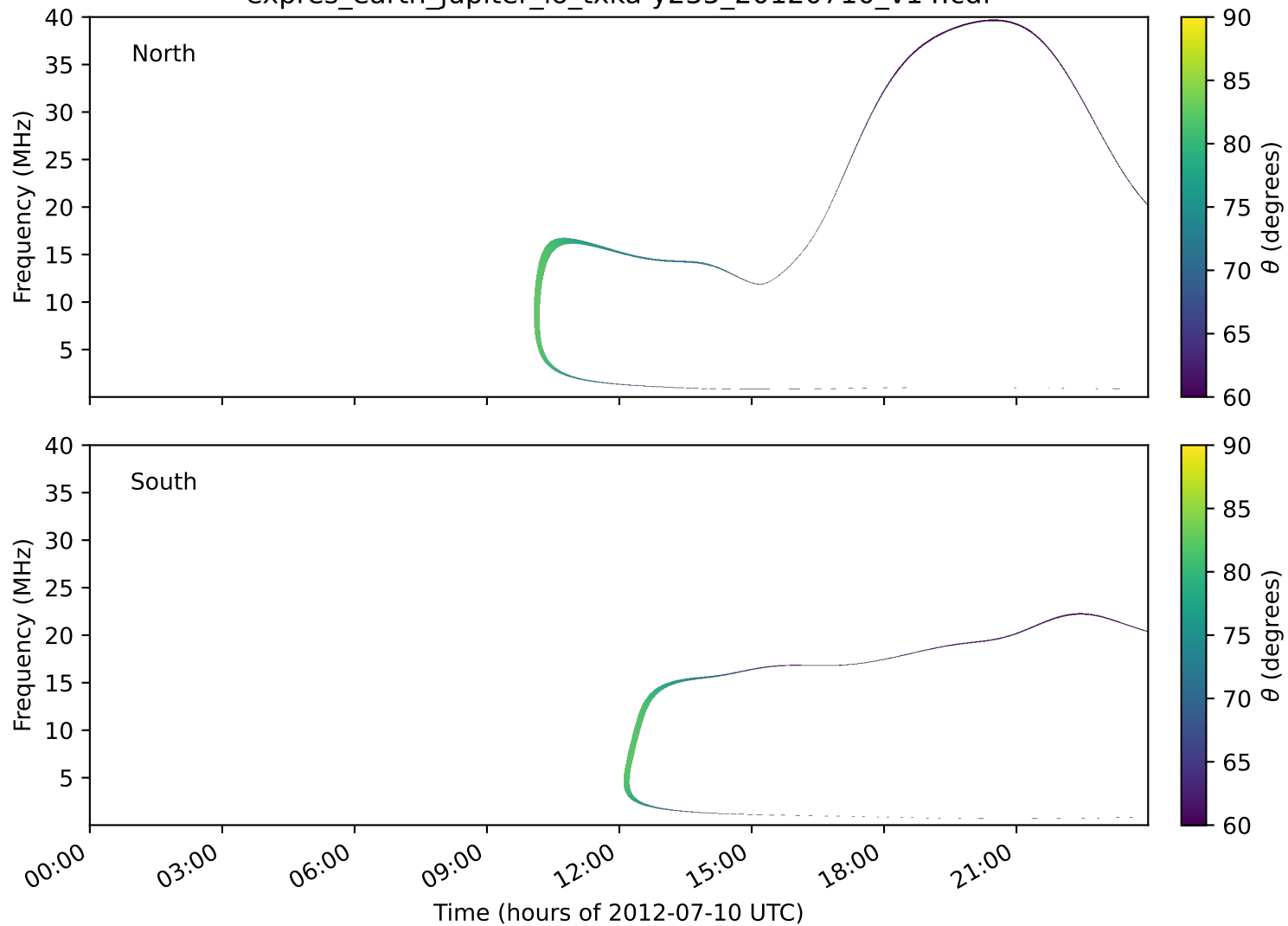
expres_earth_jupiter_io_txka-y235_20120710_v14.cdf
