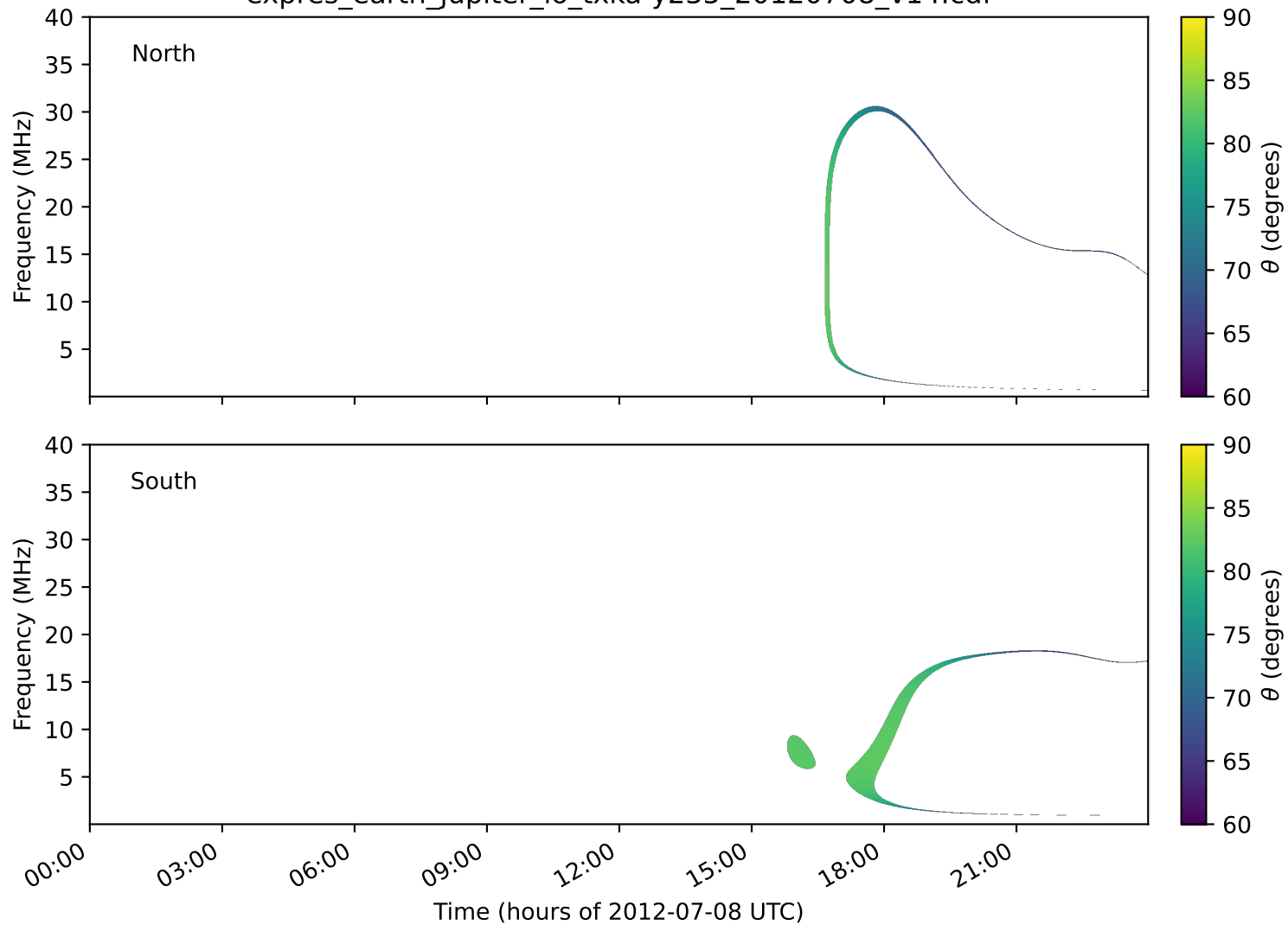
expres_earth_jupiter_io_txka-y235_20120708_v14.cdf
