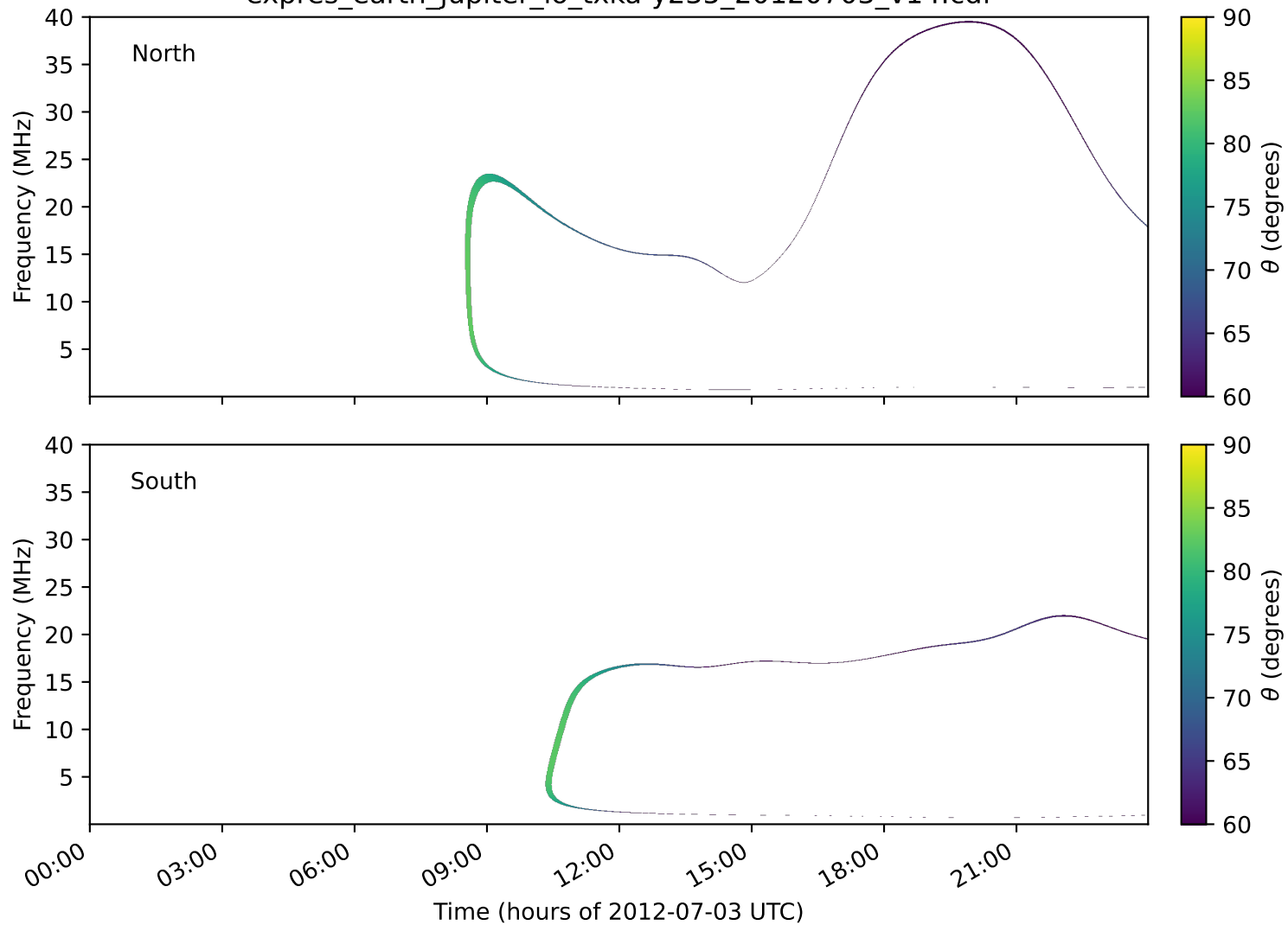
expres_earth_jupiter_io_txka-y235_20120703_v14.cdf
