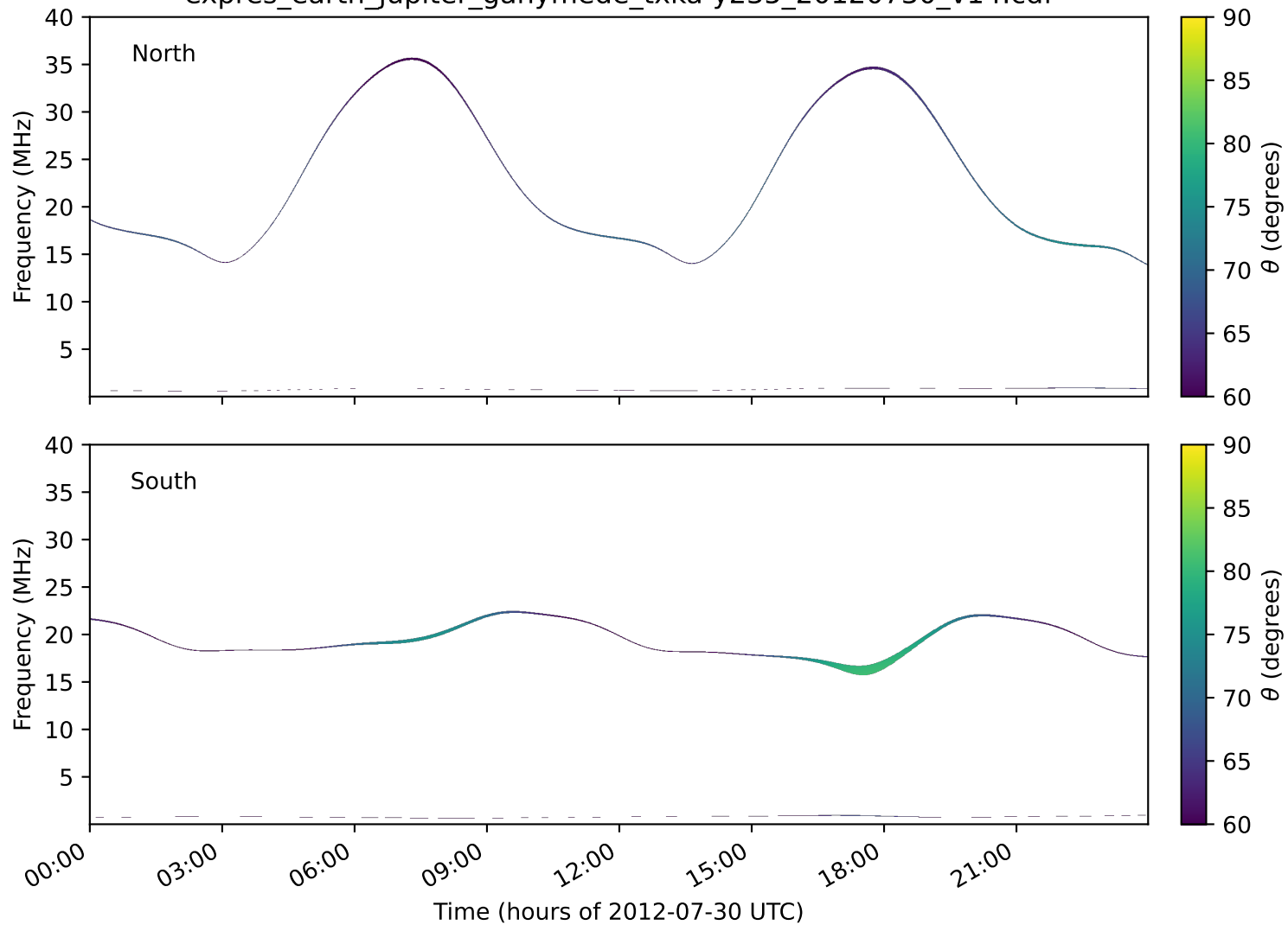
expres_earth_jupiter_ganymede_txka-y235_20120730_v14.cdf
