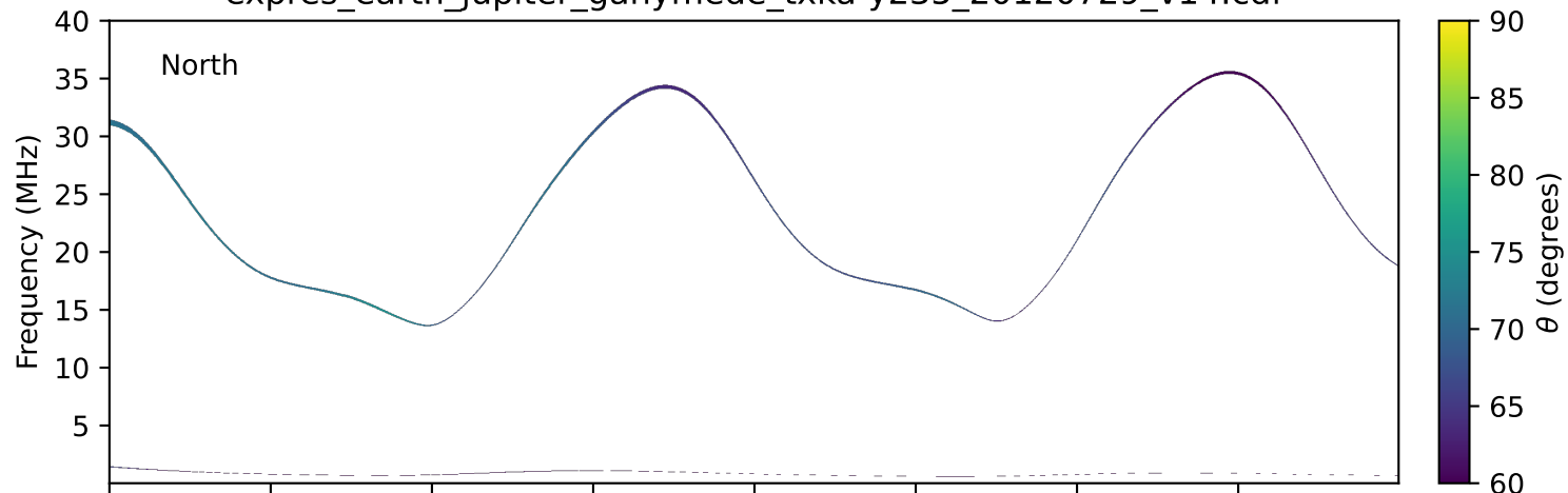
expres_earth_jupiter_ganymede_txka-y235_20120729_v14.cdf
