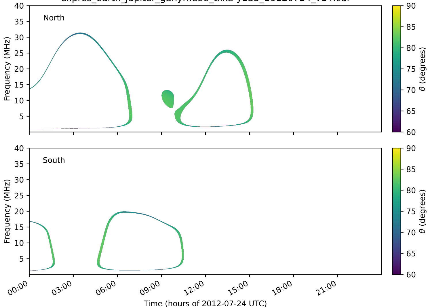
expres_earth_jupiter_ganymede_txka-y235_20120724_v14.cdf
