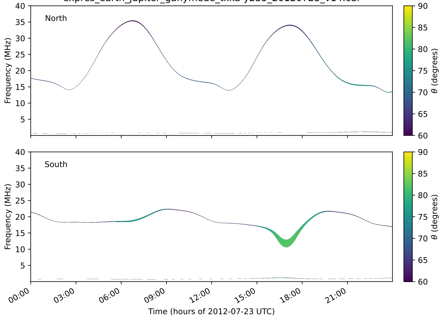
expres_earth_jupiter_ganymede_txka-y235_20120723_v14.cdf
