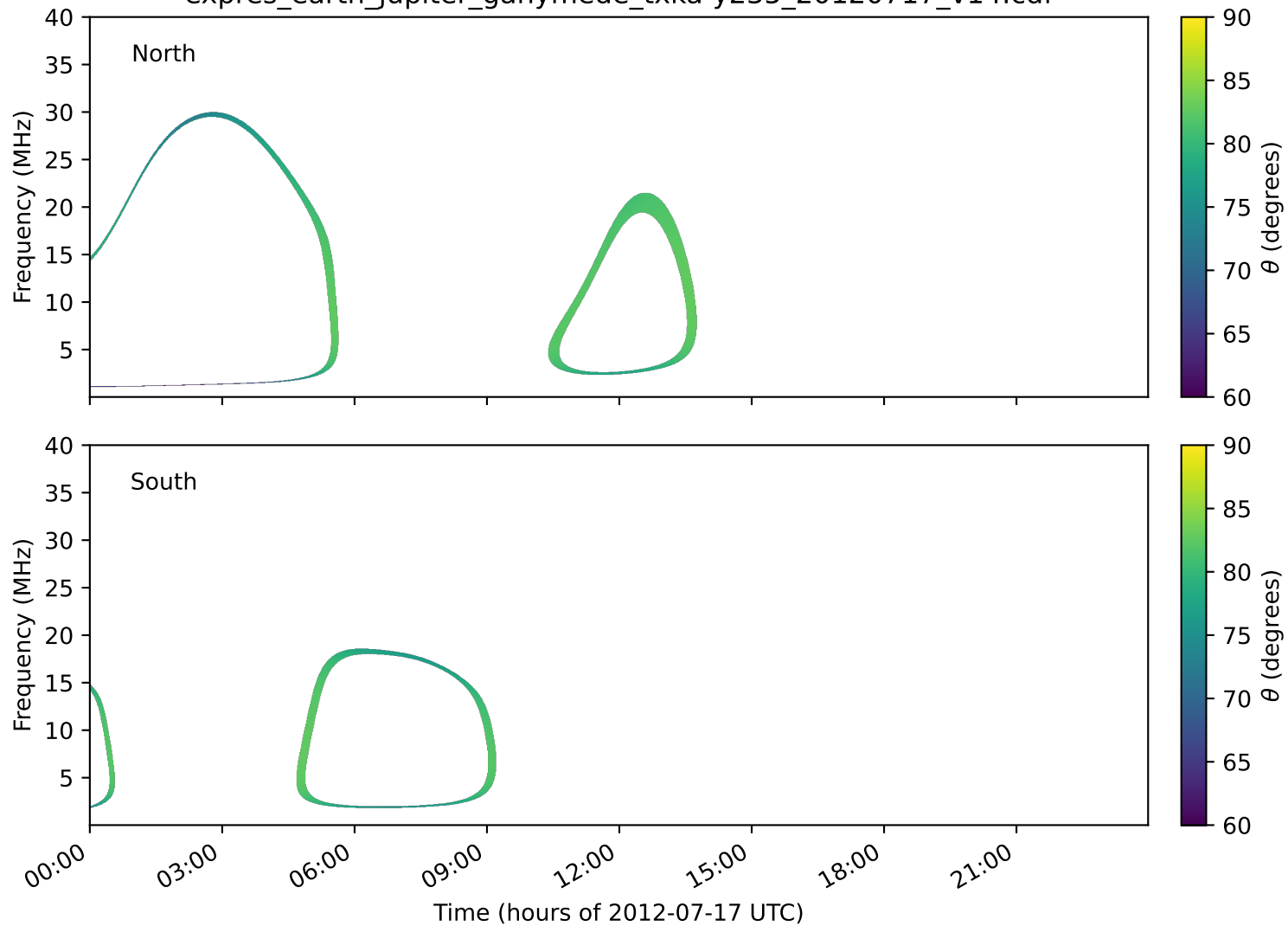
expres_earth_jupiter_ganymede_txka-y235_20120717_v14.cdf
