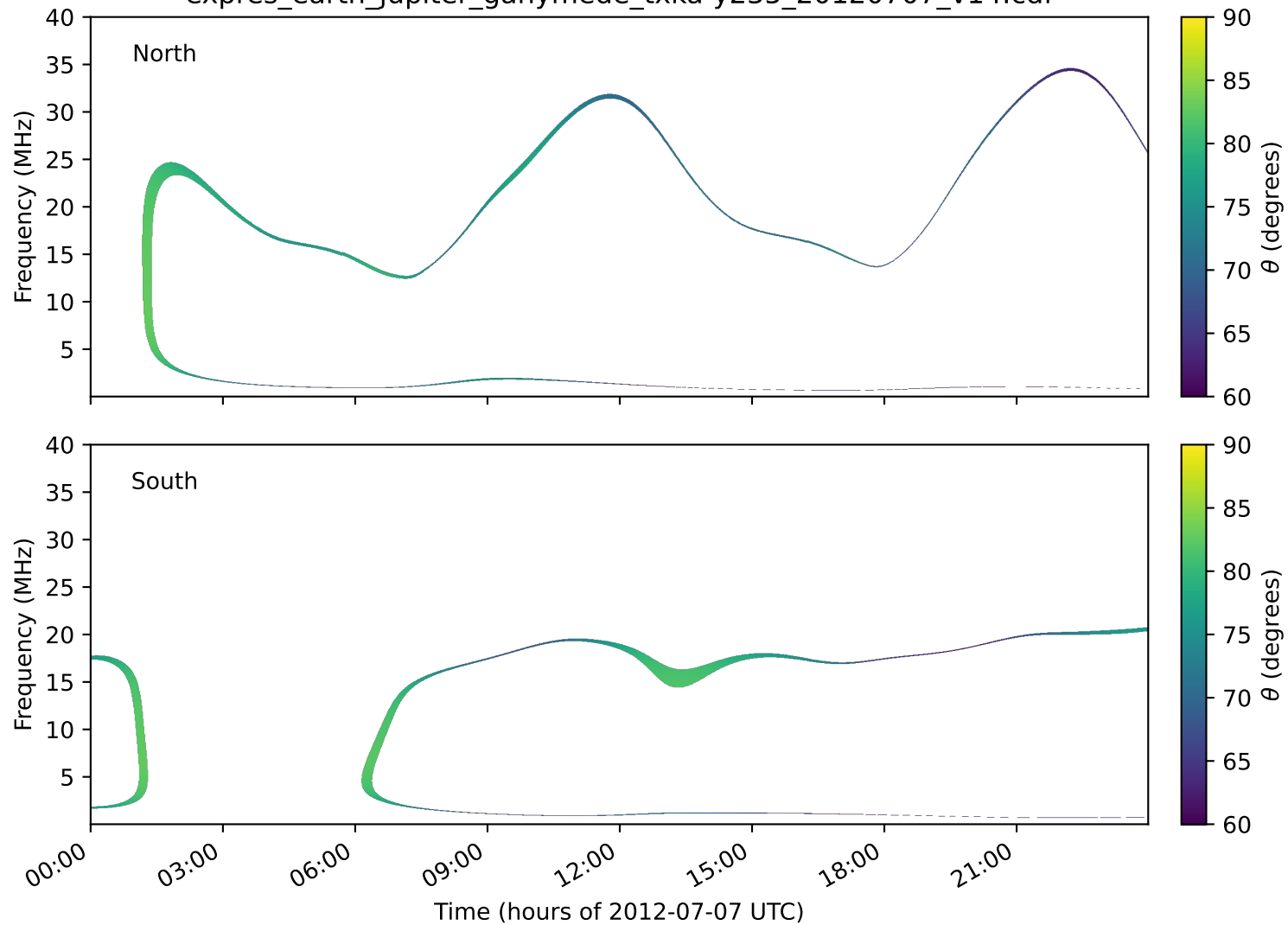
expres_earth_jupiter_ganymede_txka-y235_20120707_v14.cdf
