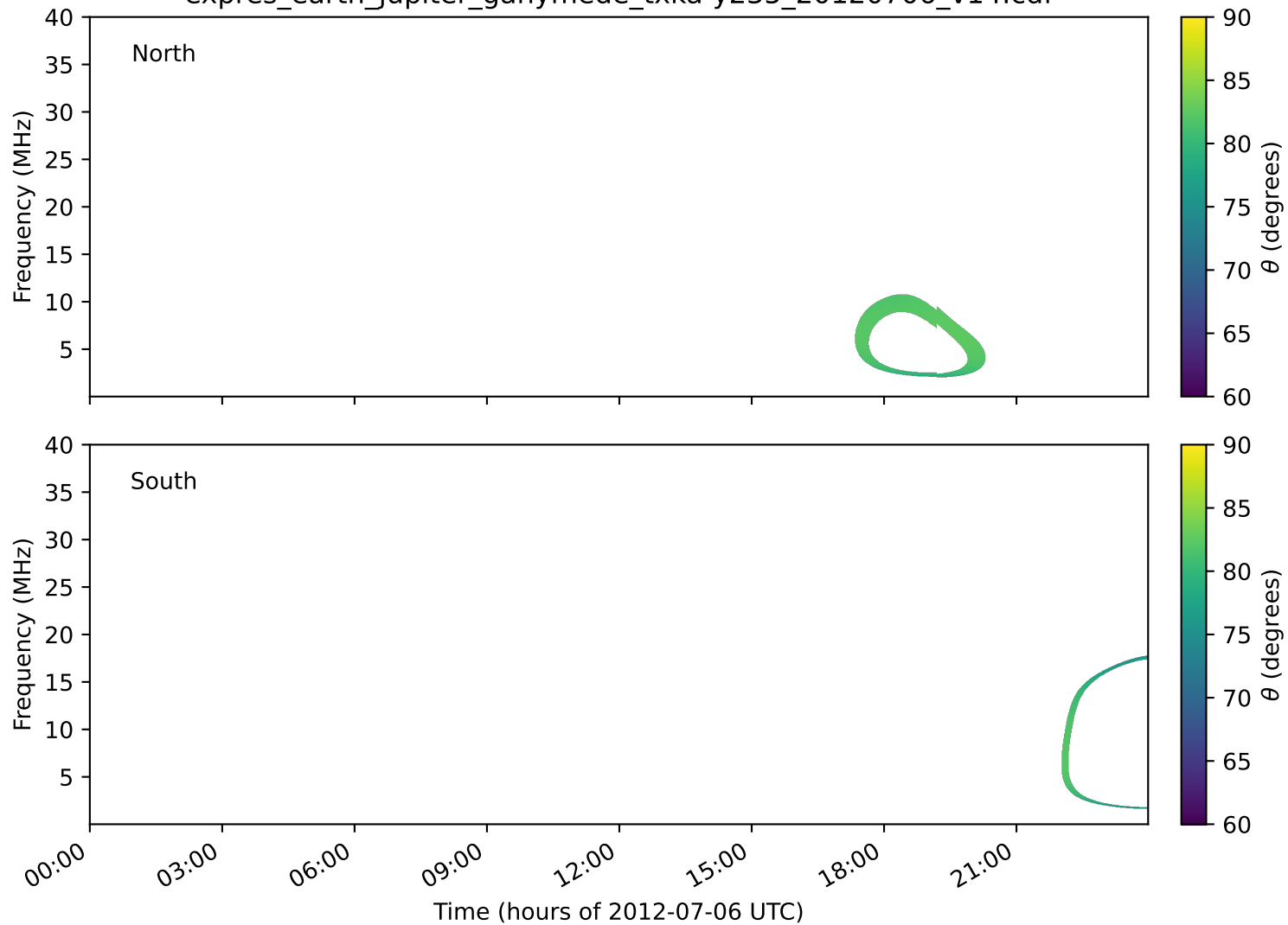
expres_earth_jupiter_ganymede_txka-y235_20120706_v14.cdf
