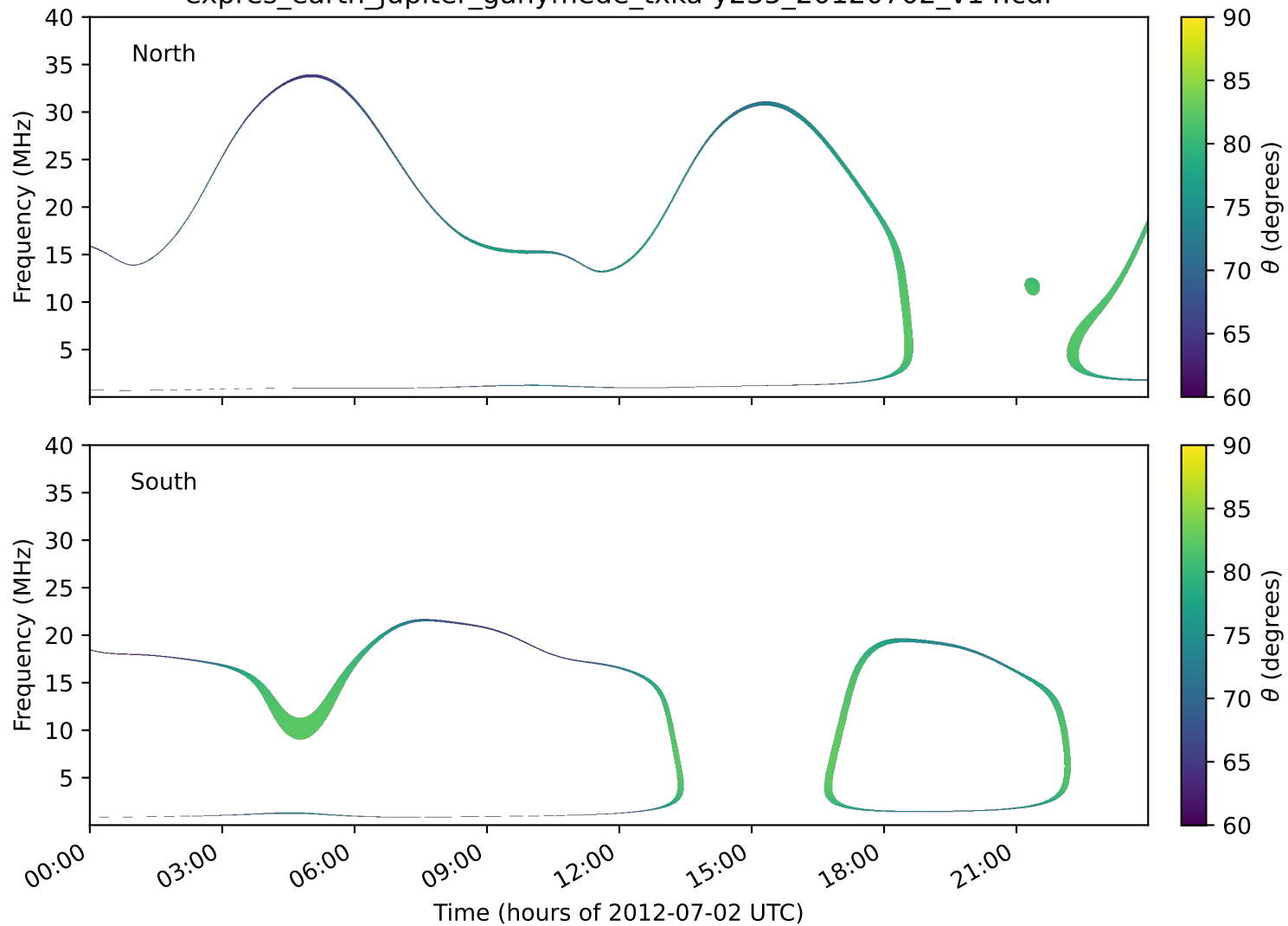
expres_earth_jupiter_ganymede_txka-y235_20120702_v14.cdf
