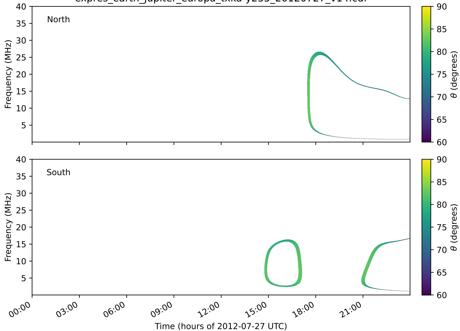
expres_earth_jupiter_europa_txka-y235_20120727_v14.cdf
