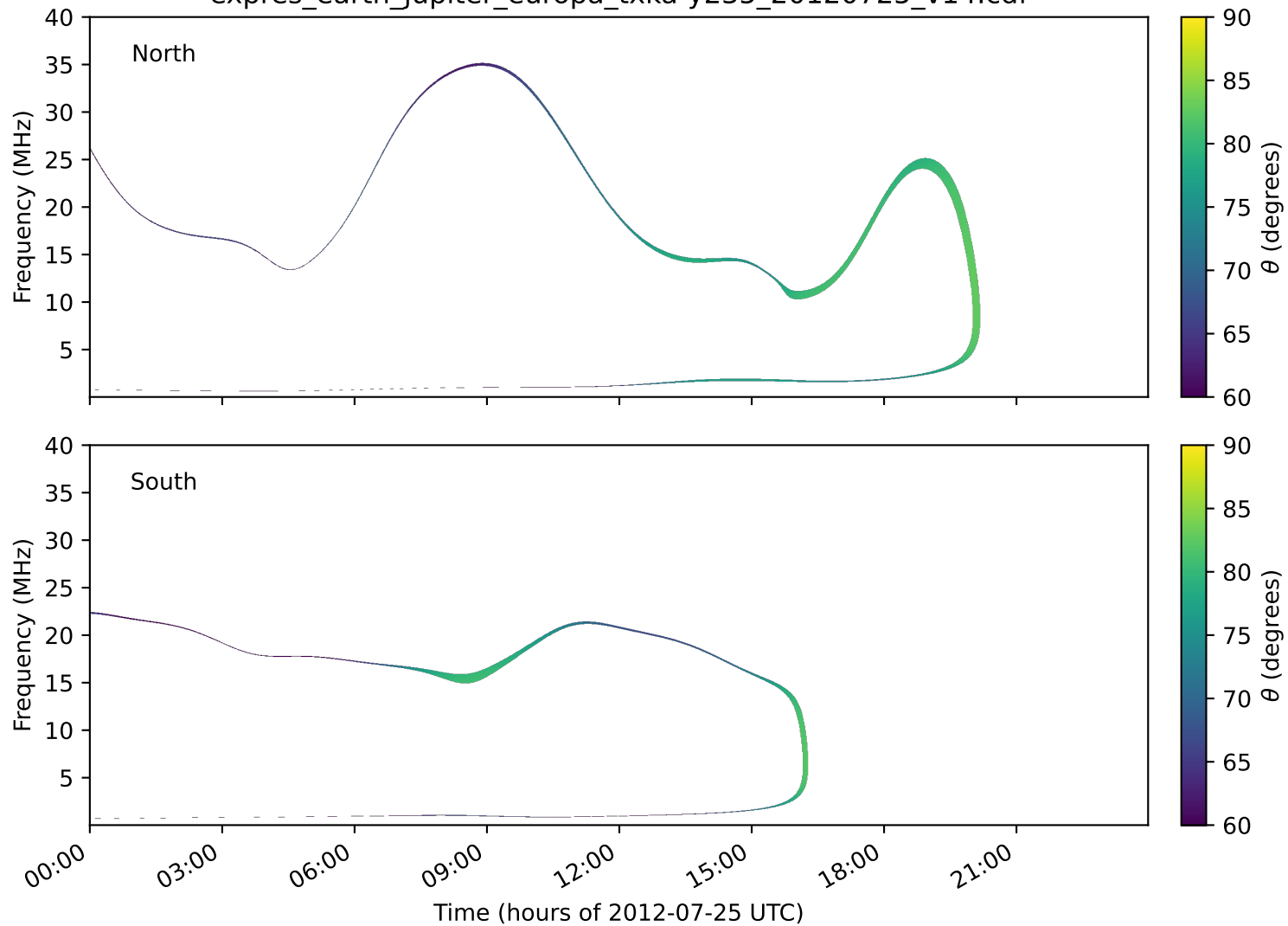
expres_earth_jupiter_europa_txka-y235_20120725_v14.cdf
