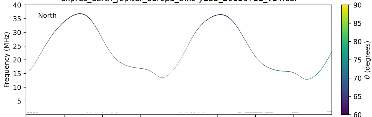
expres_earth_jupiter_europa_txka-y235_20120721_v14.cdf
