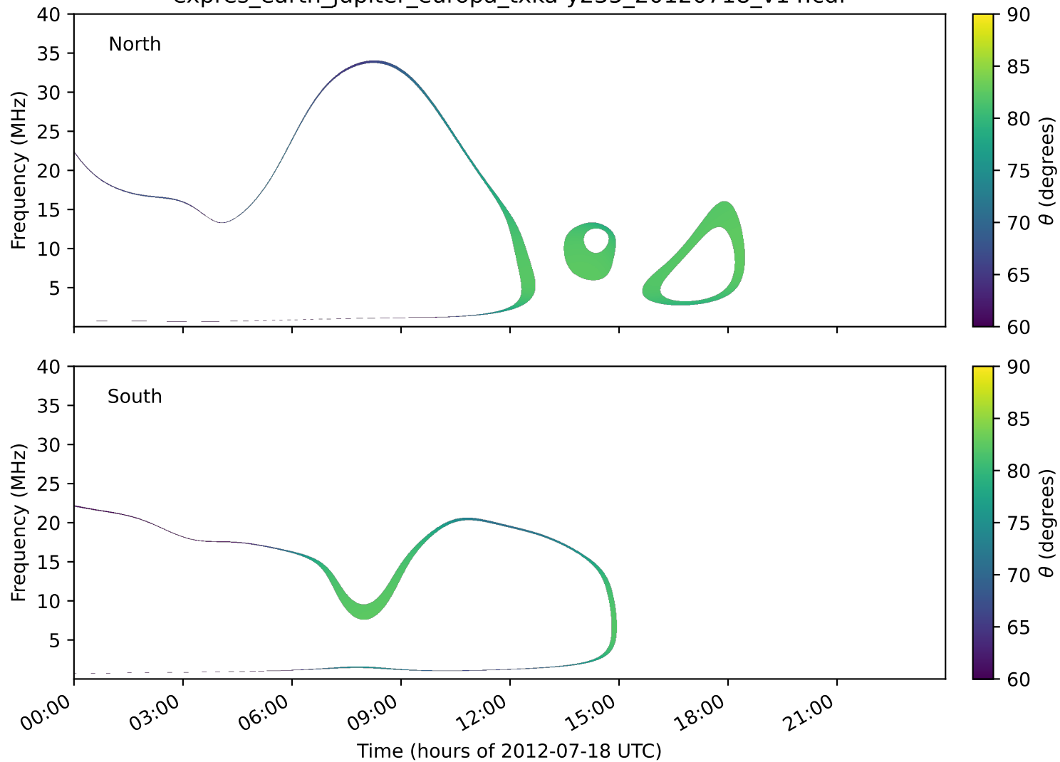
expres_earth_jupiter_europa_txka-y235_20120718_v14.cdf
