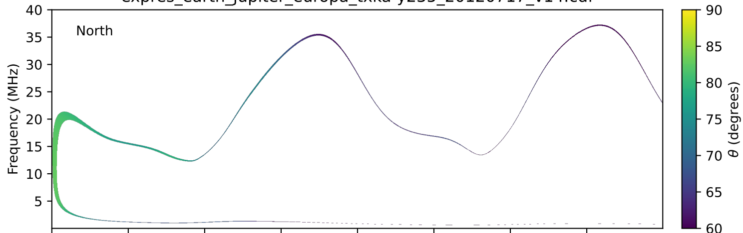
expres_earth_jupiter_europa_txka-y235_20120717_v14.cdf
