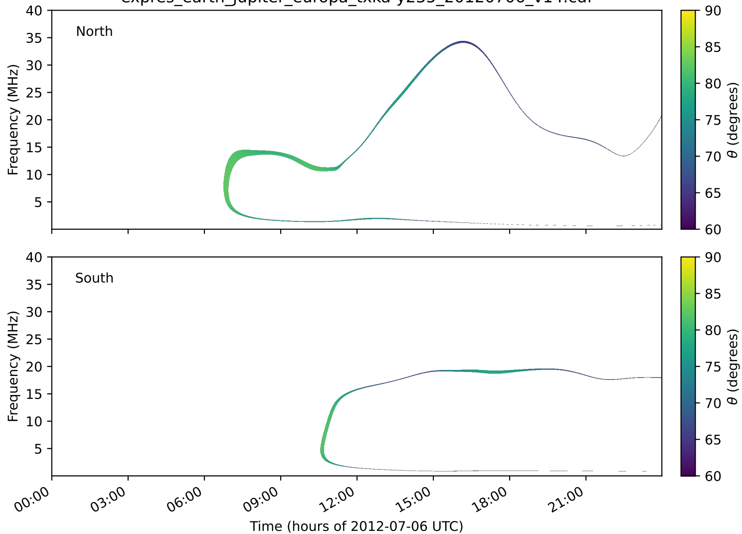
expres_earth_jupiter_europa_txka-y235_20120706_v14.cdf
