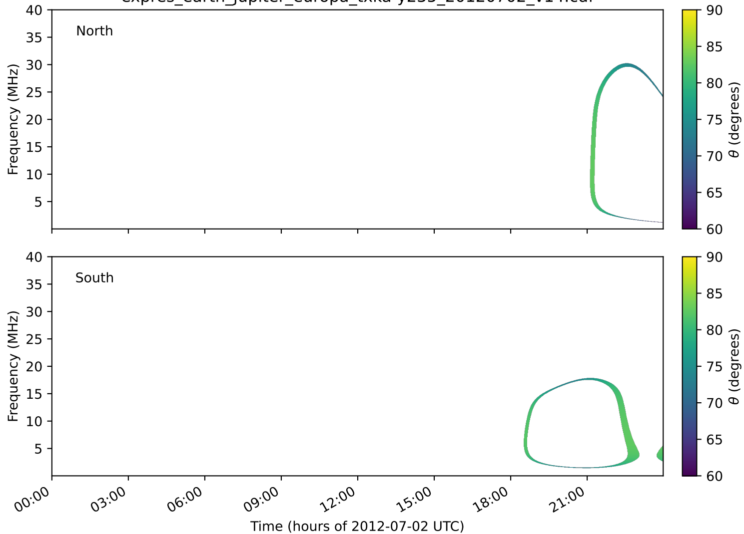
expres_earth_jupiter_europa_txka-y235_20120702_v14.cdf
