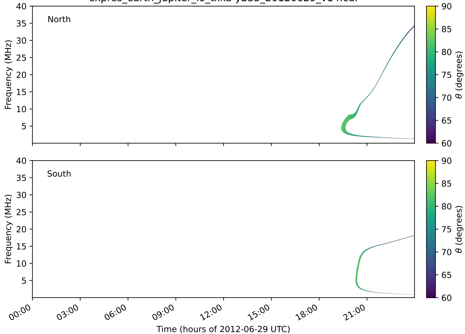
expres_earth_jupiter_io_txka-y235_20120629_v14.cdf
