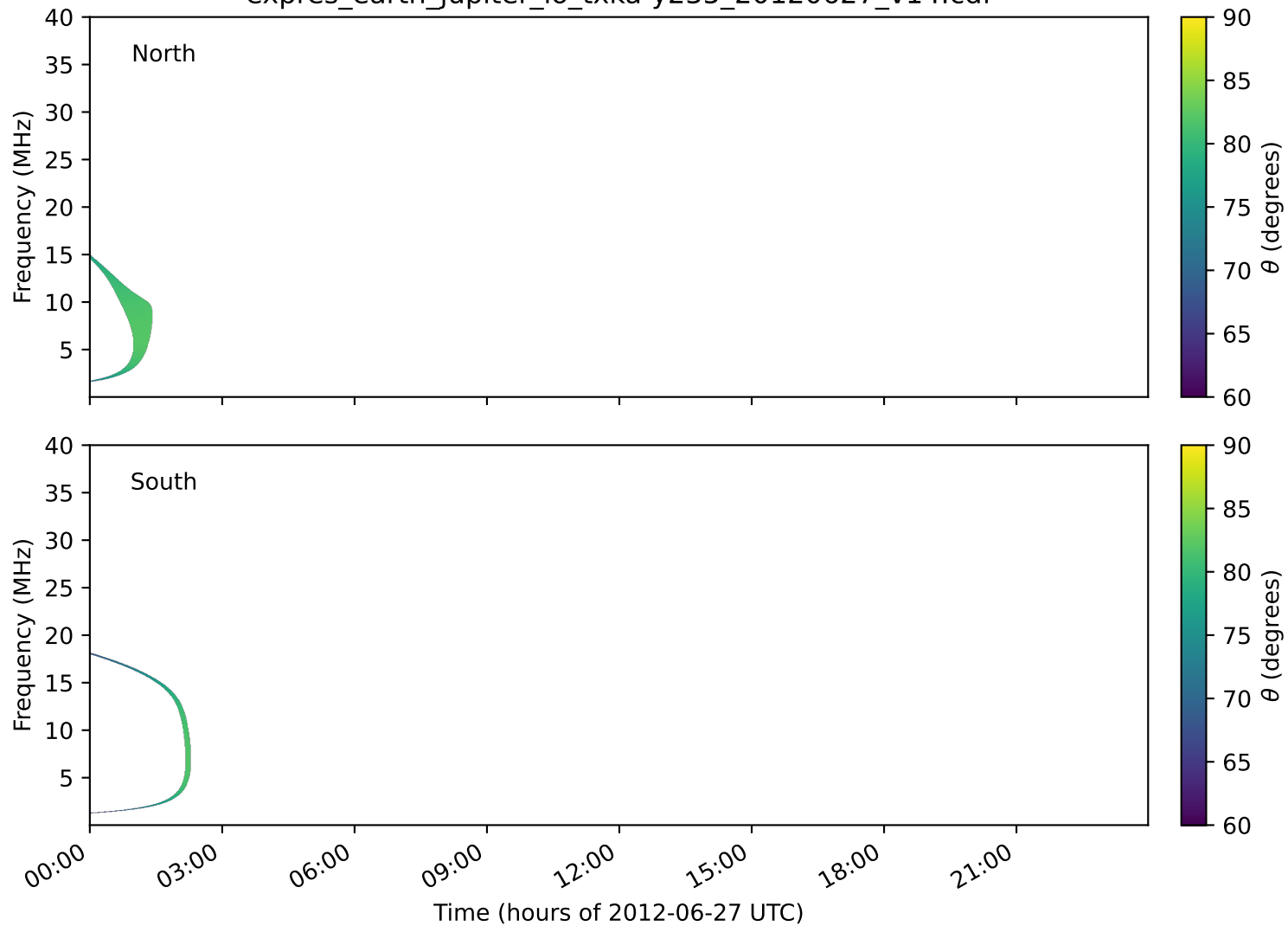
expres_earth_jupiter_io_txka-y235_20120627_v14.cdf
