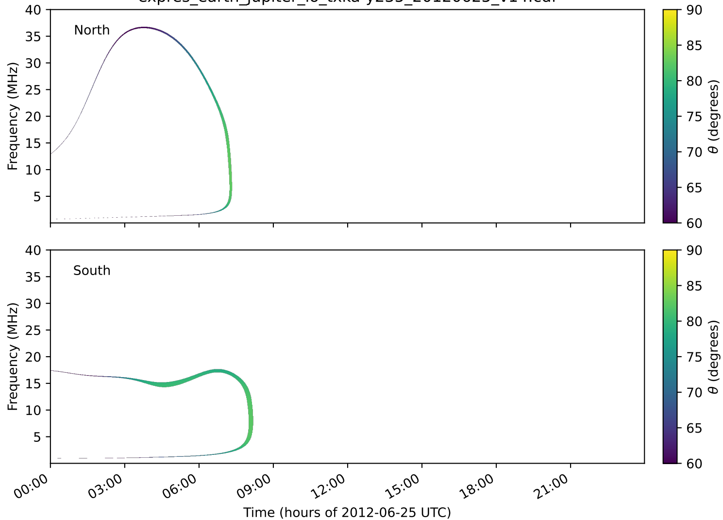
expres_earth_jupiter_io_txka-y235_20120625_v14.cdf
