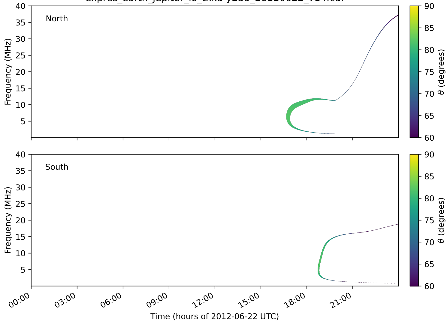
expres_earth_jupiter_io_txka-y235_20120622_v14.cdf
