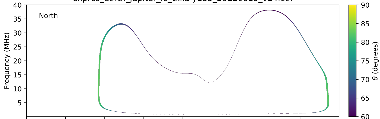
expres_earth_jupiter_io_txka-y235_20120619_v14.cdf
