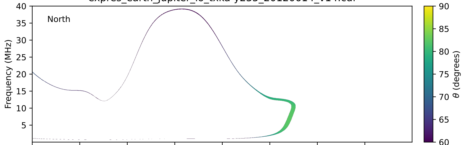
expres_earth_jupiter_io_txka-y235_20120614_v14.cdf
