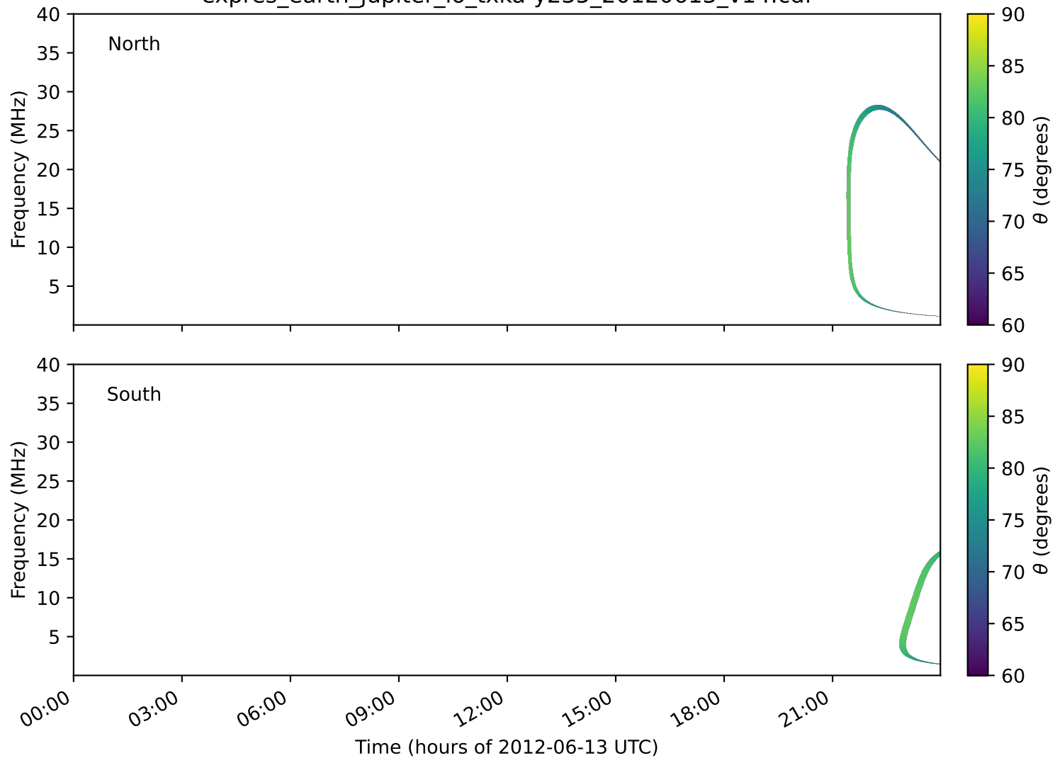
expres_earth_jupiter_io_txka-y235_20120613_v14.cdf
